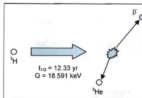
Figure 16: Virtually all helium-3 in present worldwide stores has been produced as a product of tritium \beta -decay.
