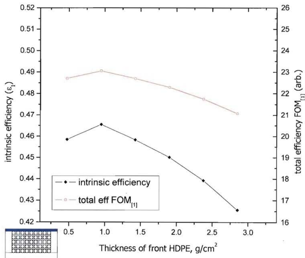
Figure 34: Efficiency parameters vs. front face-thickness for the semi-infinite
