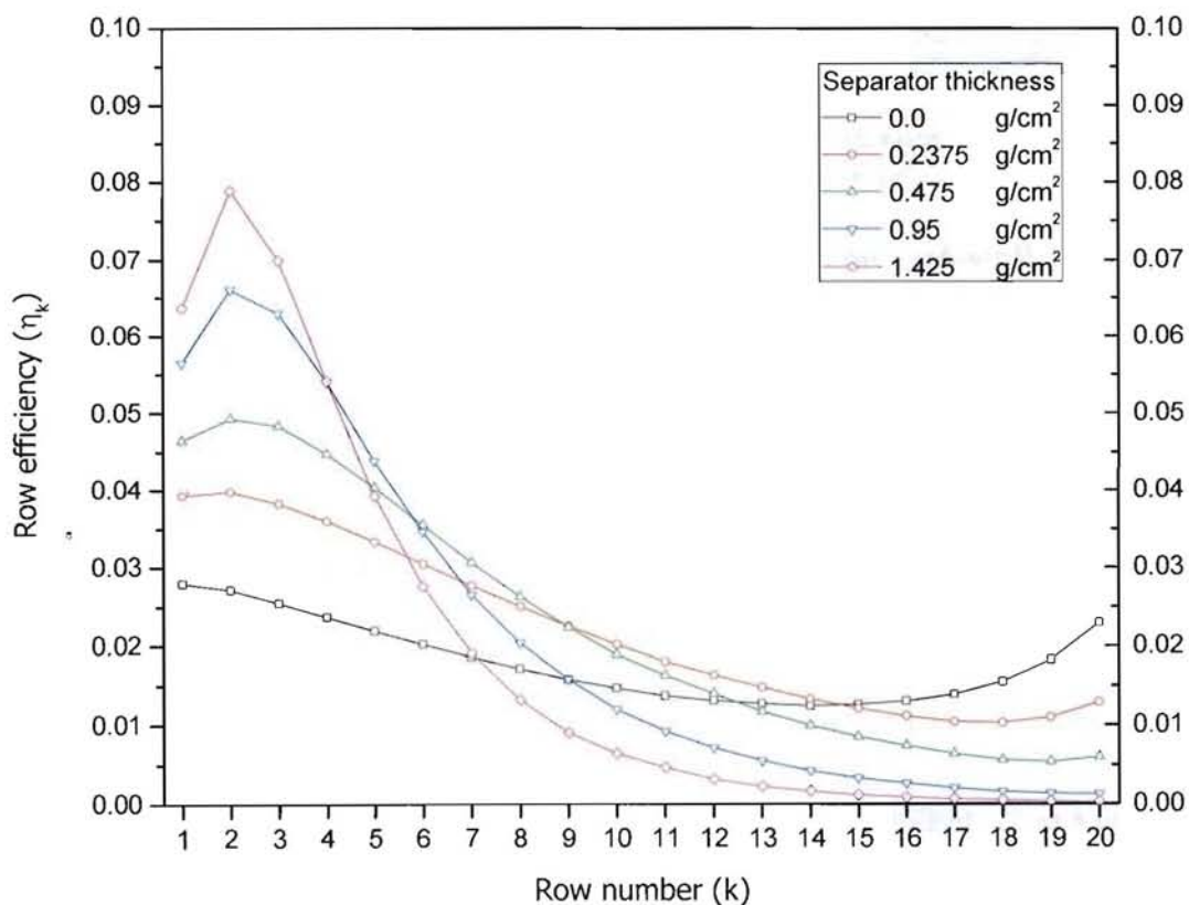
Figure 37: Row-sum efficiencies of the semi-infinite ANDY detector for several
