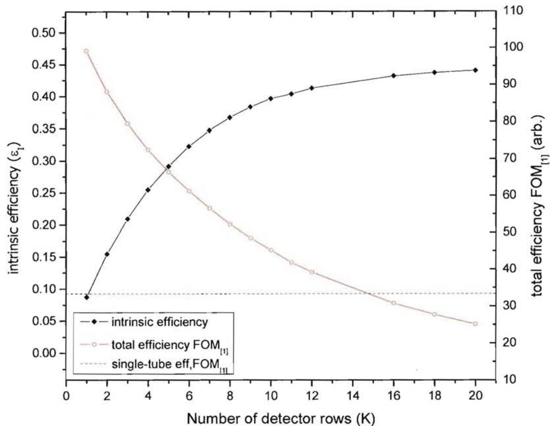
Figure 38: Efficiency parameters versus number of detectors rows for a uniform rectangular ANDY detector. The lattice parameters were identical in each case: 9.5 g/cm 2 in the top, bottom, rear, and outer sides; 1.425 g/cm 2 in front; and 0.7125 g/cm 2 in the separators and sidewalls. The results from the single high-pressure tube of section 4.2.1 appear as a dashed line for comparison; the two y-axes were aligned so the efficiency and figure-of-merit for the single-tube coincide. The statistical error bars are less than 1%.
