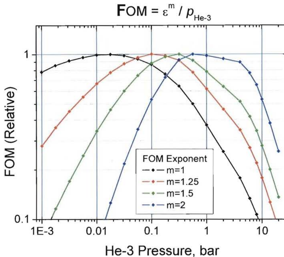
Figure 8: Efficiency of a 1" x 12" cylindrical He-3 detector versus He-3 partial pressure in terms of cost efficiency. The efficiency figure-of-merit (FOM) used in cost efficiency is defined as weighted efficiency per unit He-3 gas. The exponential weighting factor m controls the relative emphasis between efficiency and amount of gas used. Statistical error bars are less than 1%.
