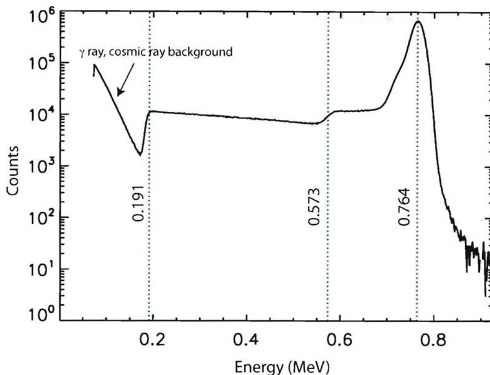
Figure 4: Energy spectrum of 2"-dia. x 48"-long detector containing 200-mbar He-3 and 800-mbar proportional gas. Neutron counts appear above 191-keV and background counts from gamma-rays, cosmic rays, and electronic noise appear at lower energies, as indicated. Wall effects from both p (573 keV) and T (191 keV) daughters are clearly resolved.
